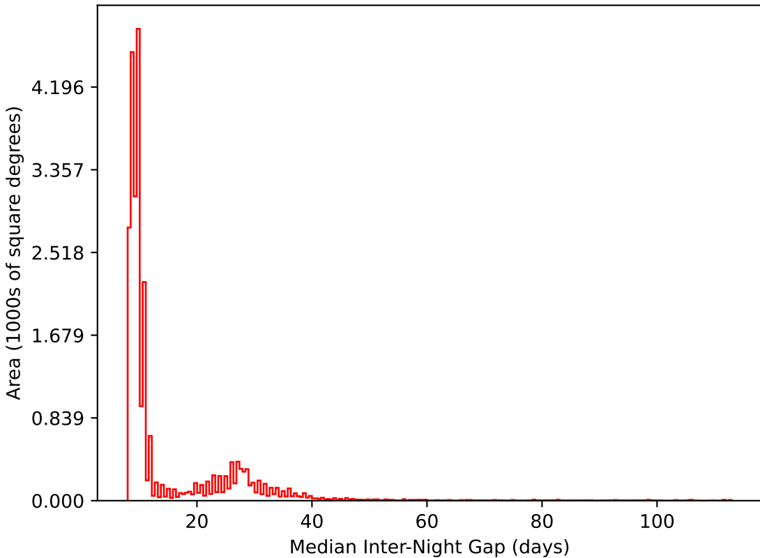
noroll_v3.4_10yrs All sky i band: Median Inter-Night Gap
