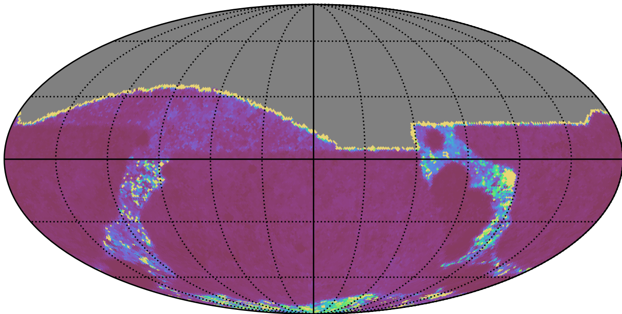
noroll_v3.4_10yrs All sky g band: Median Inter-Night Gap
