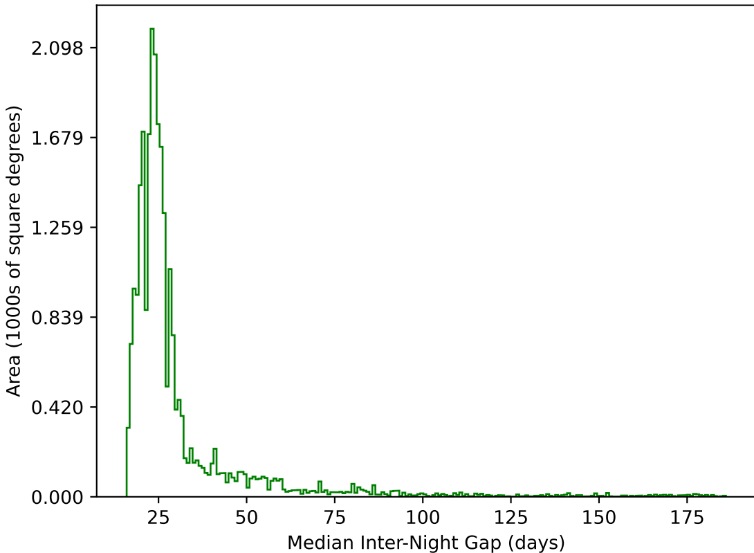
noroll_v3.4_10yrs All sky g band: Median Inter-Night Gap
