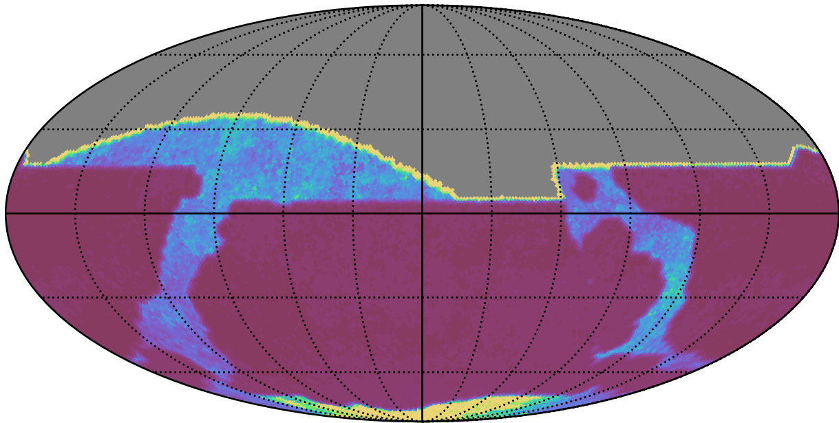
noroll_v3.4_10yrs All sky all bands: Median Inter-Night Gap
