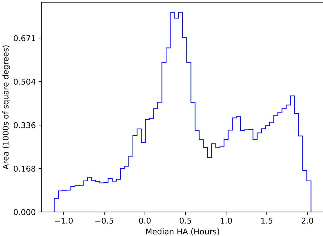
noroll_v3.4_10yrs WFD z band: Median HA
