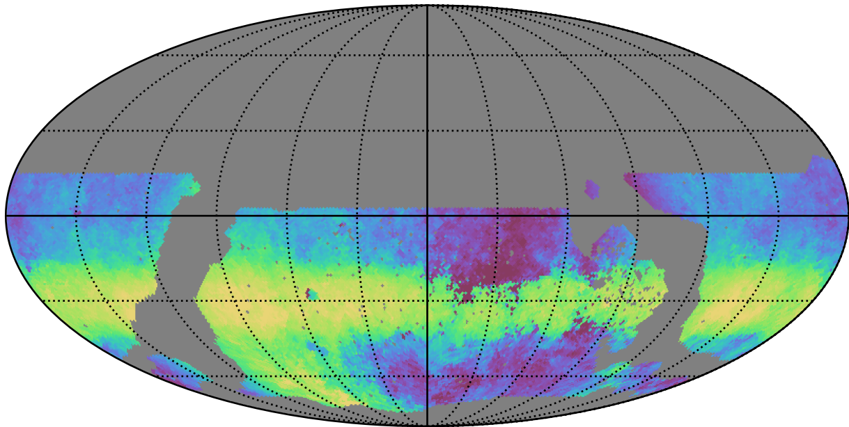
noroll_v3.4_10yrs WFD y band: Median HA
