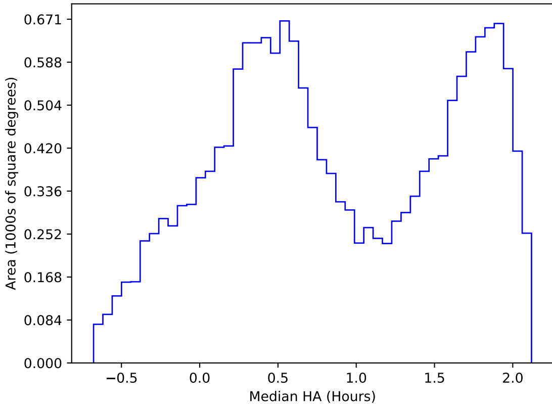
noroll_v3.4_10yrs WFD y band: Median HA
