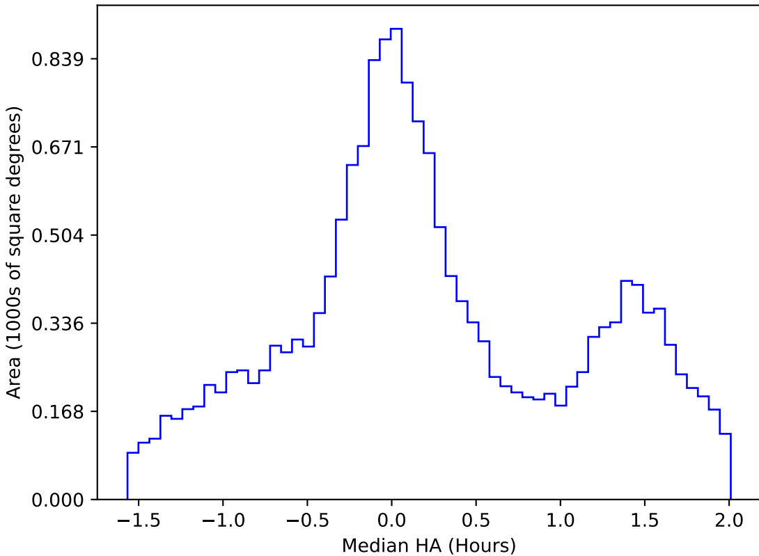
noroll_v3.4_10yrs WFD u band: Median HA
