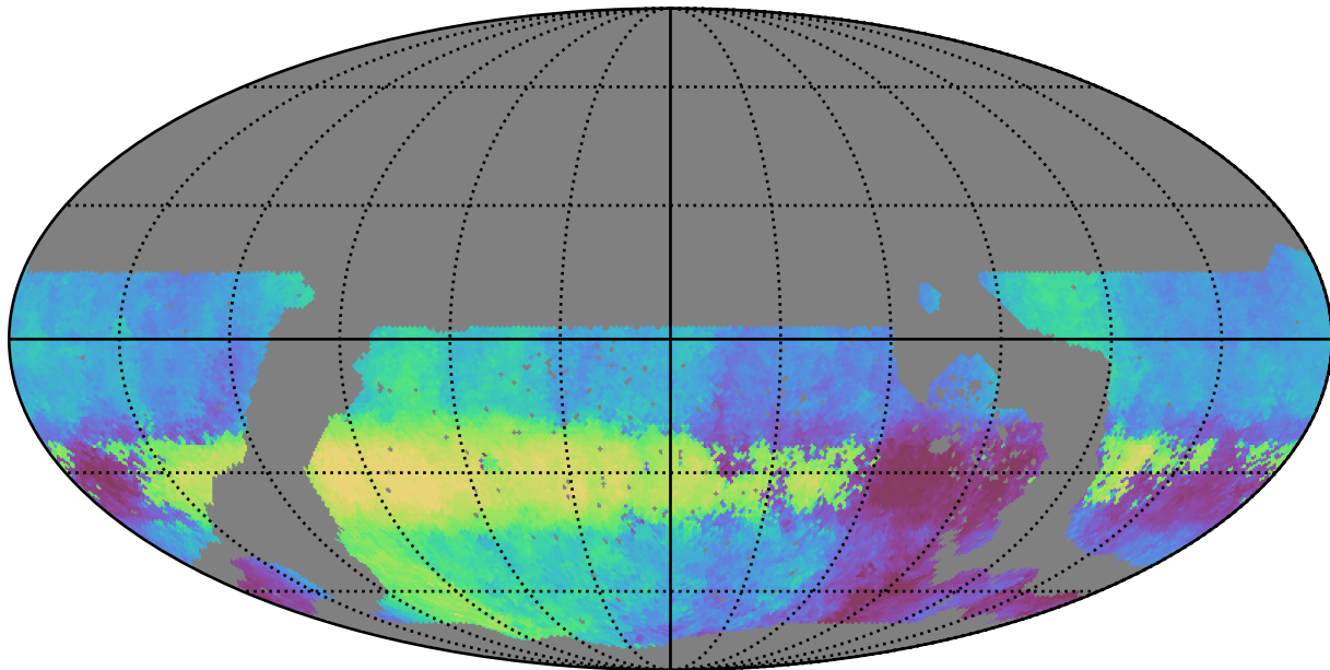
noroll_v3.4_10yrs WFD r band: Median HA
