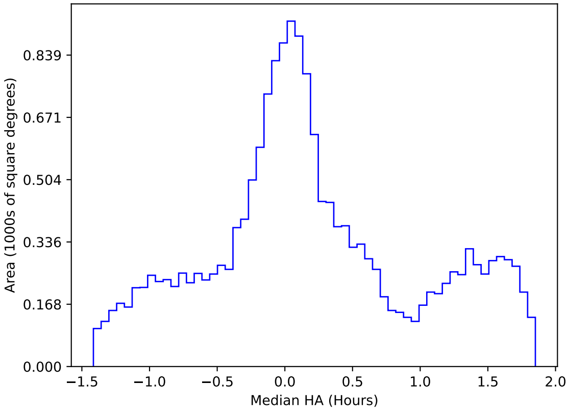
noroll_v3.4_10yrs WFD r band: Median HA
