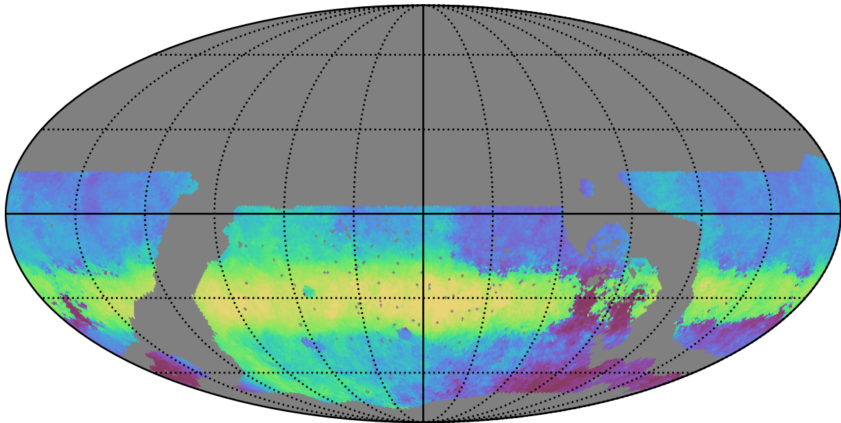
noroll_v3.4_10yrs WFD i band: Median HA
