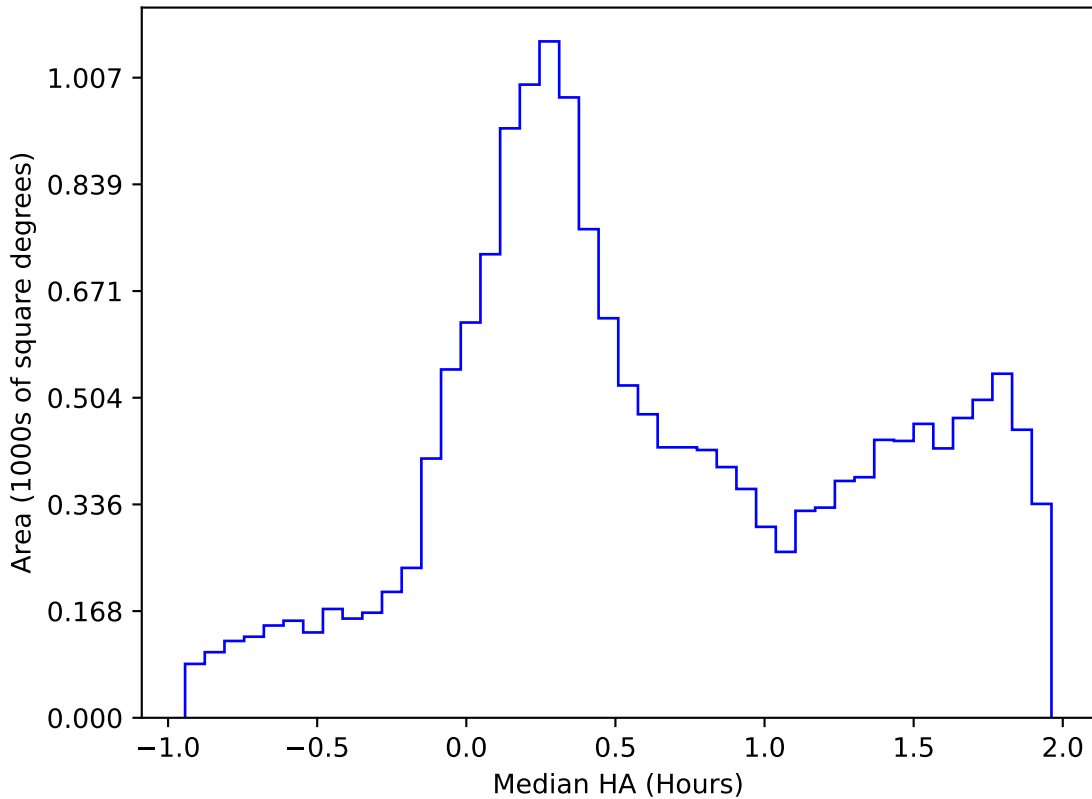
noroll_v3.4_10yrs WFD i band: Median HA
