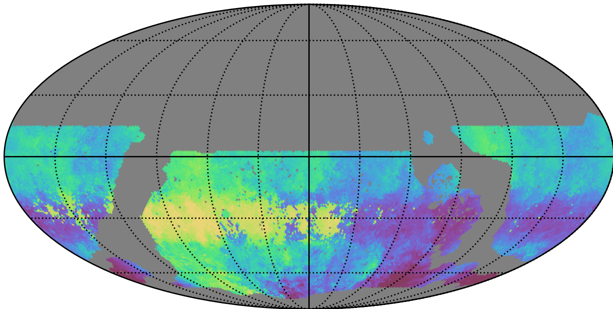
noroll_v3.4_10yrs WFD g band: Median HA
