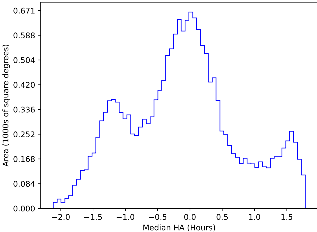
noroll_v3.4_10yrs WFD g band: Median HA
