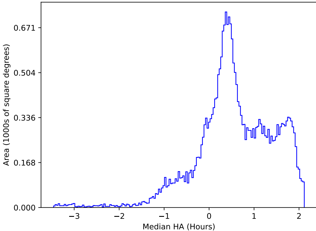
noroll_v3.4_10yrs All sky z band: Median HA
