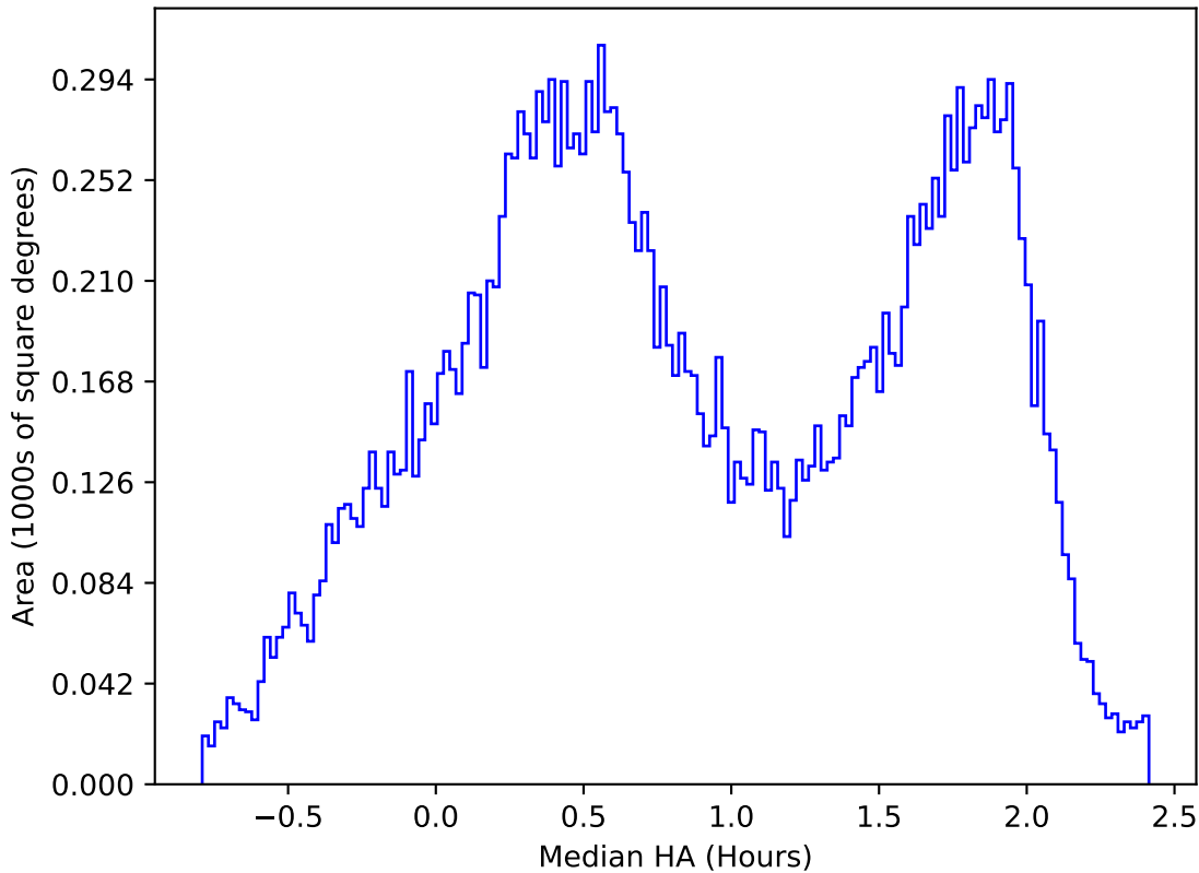
noroll_v3.4_10yrs All sky y band: Median HA
