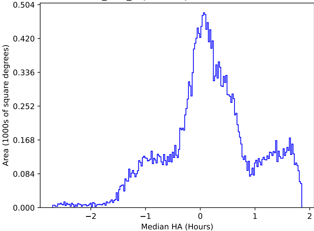
noroll_v3.4_10yrs All sky r band: Median HA
