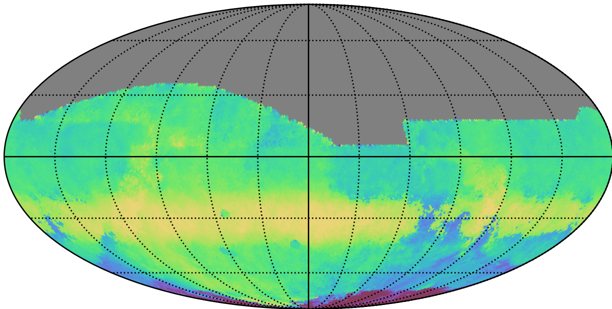
noroll_v3.4_10yrs All sky i band: Median HA
