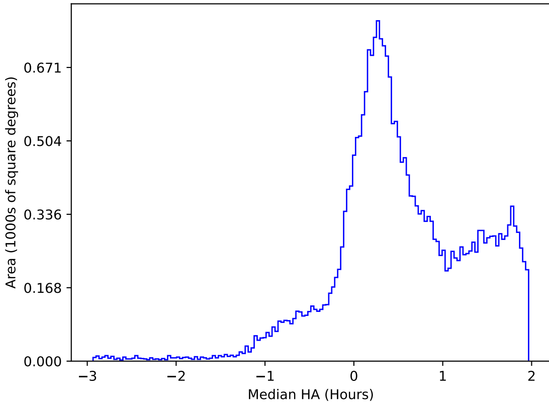
noroll_v3.4_10yrs All sky i band: Median HA
