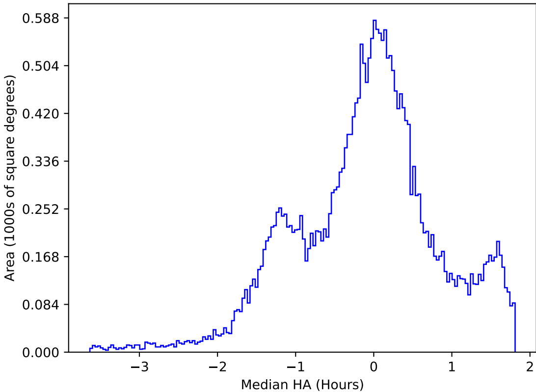
noroll_v3.4_10yrs All sky g band: Median HA
