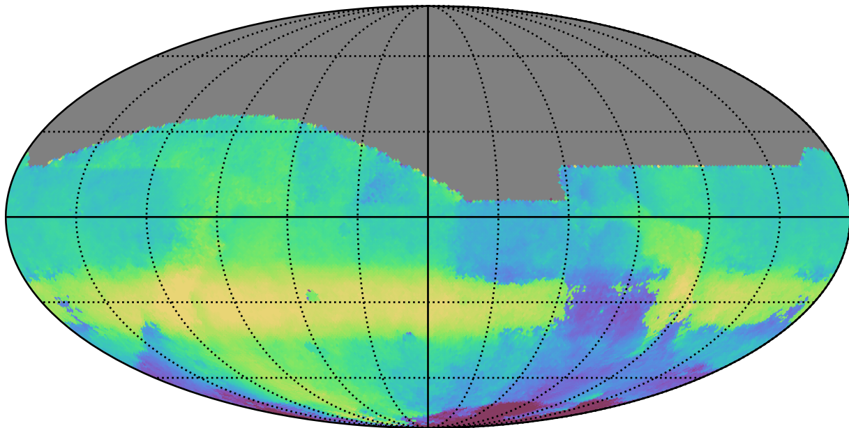
noroll_v3.4_10yrs All sky all bands: Median HA
