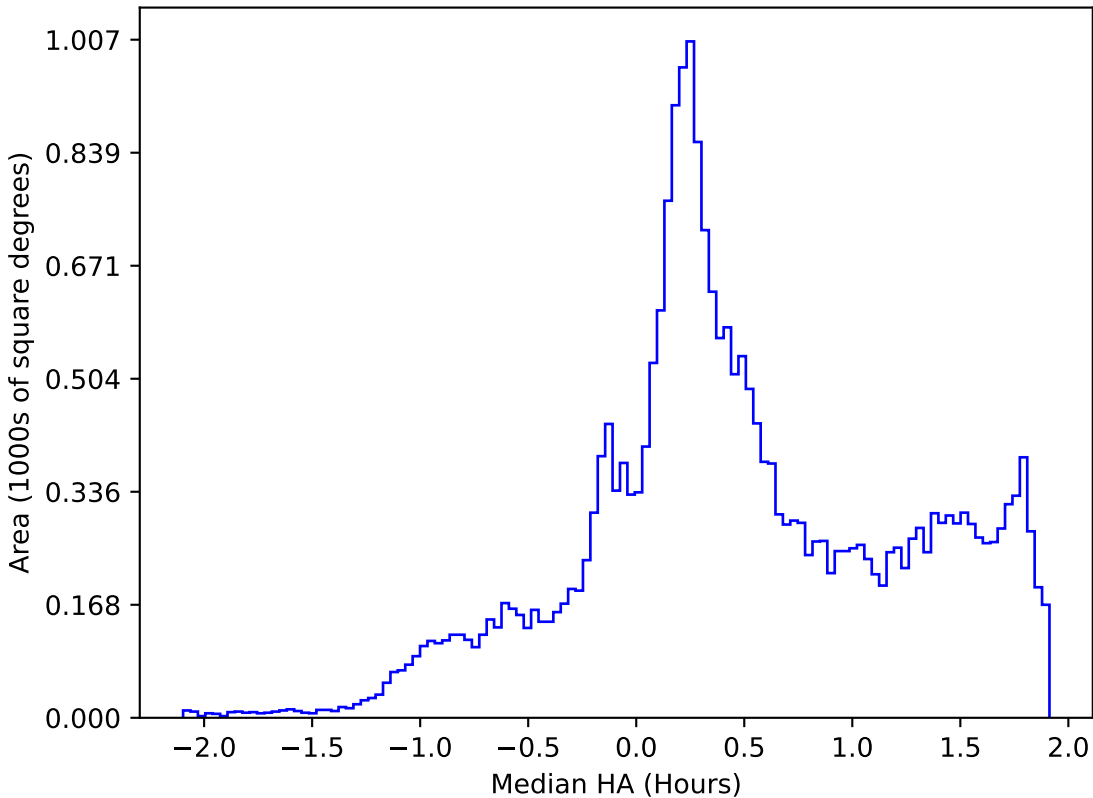
noroll_v3.4_10yrs All sky all bands: Median HA
