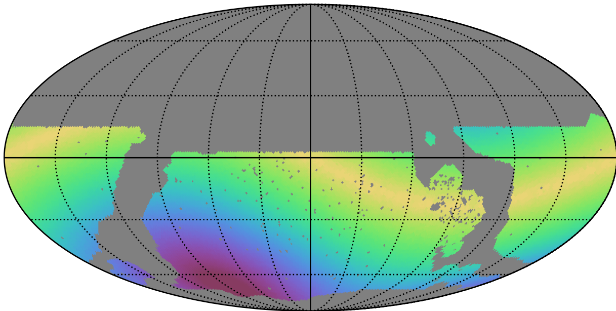
noroll_v3.4_10yrs WFD z band: Max solarElong
