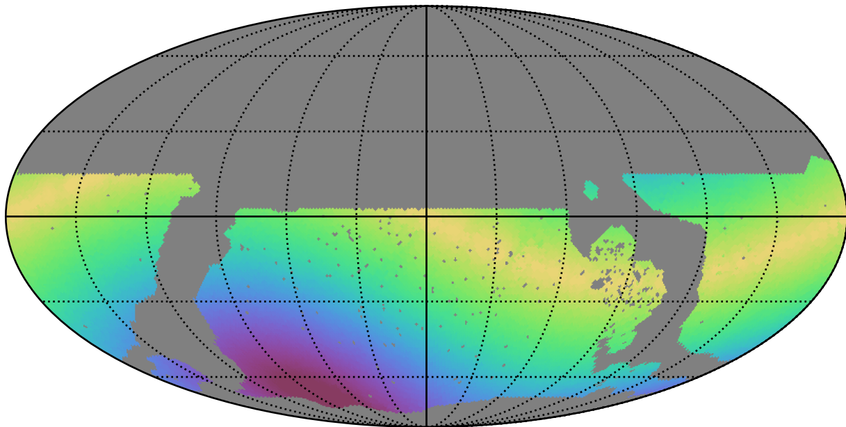
noroll_v3.4_10yrs WFD u band: Max solarElong
