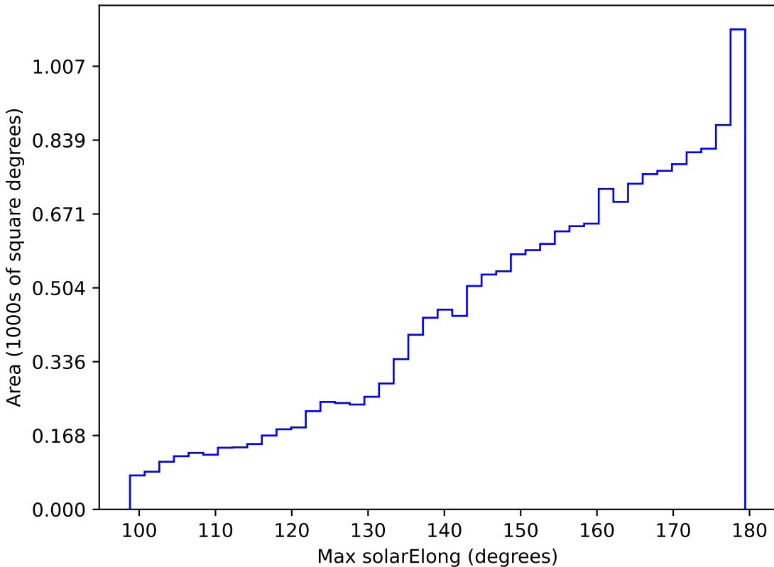
noroll_v3.4_10yrs WFD r band: Max solarElong
