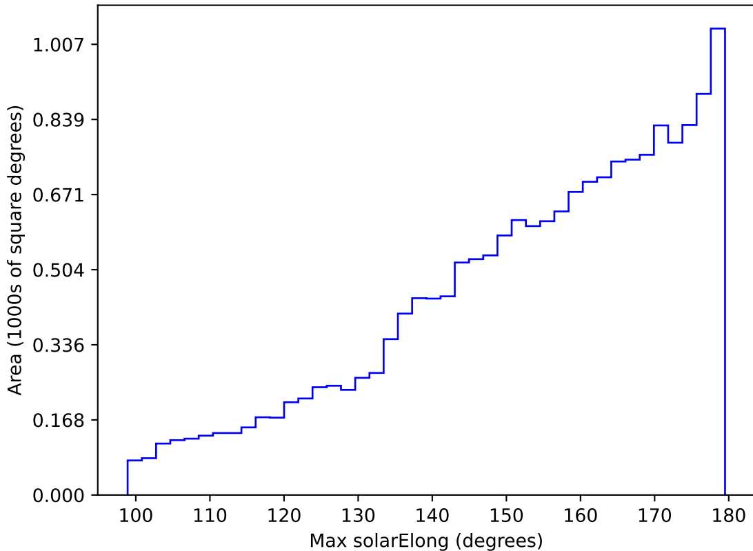
noroll_v3.4_10yrs WFD i band: Max solarElong
