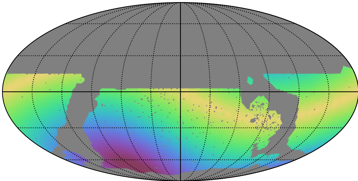
noroll_v3.4_10yrs WFD g band: Max solarElong
