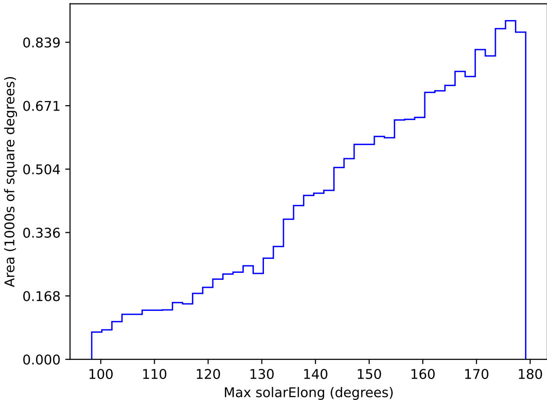
noroll_v3.4_10yrs WFD g band: Max solarElong
