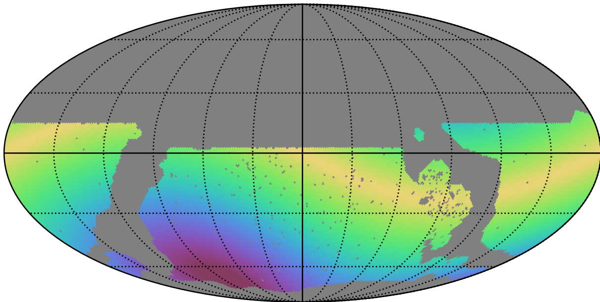
noroll_v3.4_10yrs WFD all bands: Max solarElong
