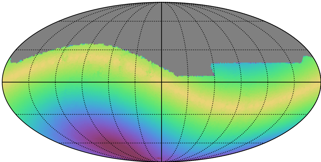
noroll_v3.4_10yrs All sky z band: Max solarElong
