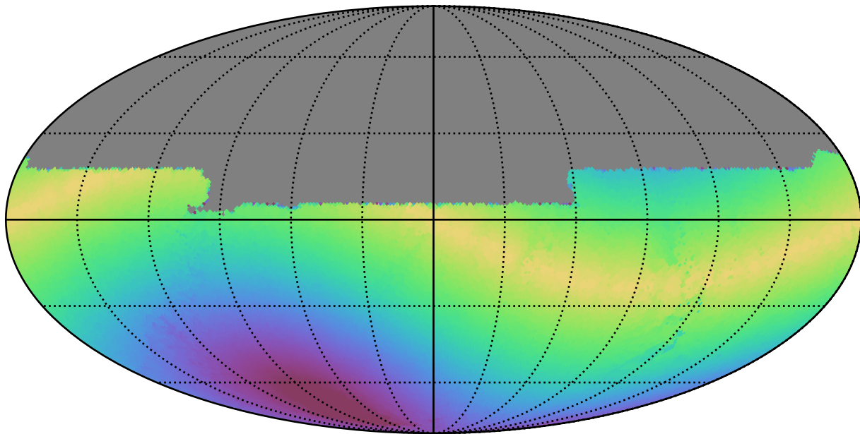
noroll_v3.4_10yrs All sky u band: Max solarElong
