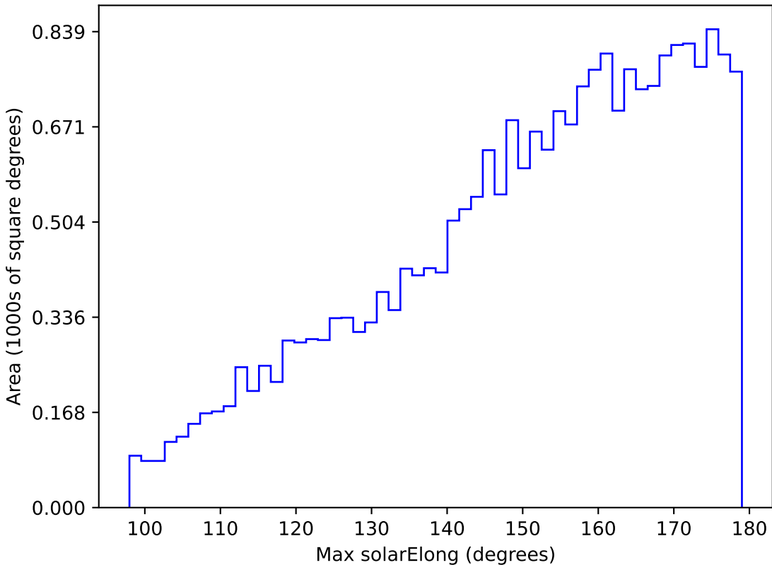
noroll_v3.4_10yrs All sky u band: Max solarElong
