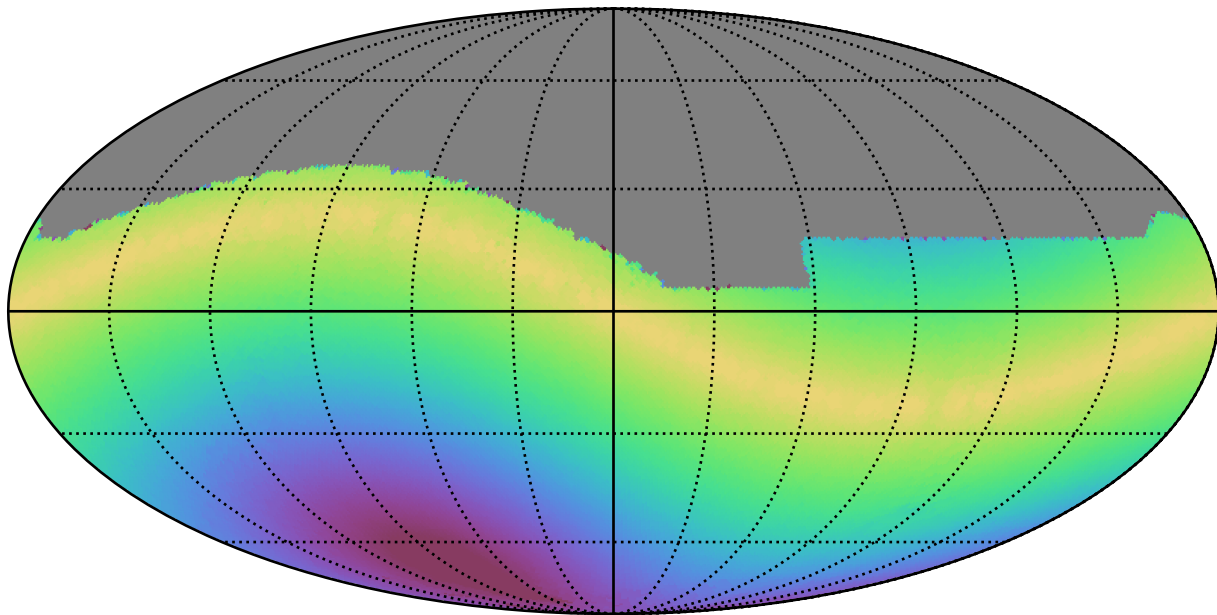
noroll_v3.4_10yrs All sky r band: Max solarElong
