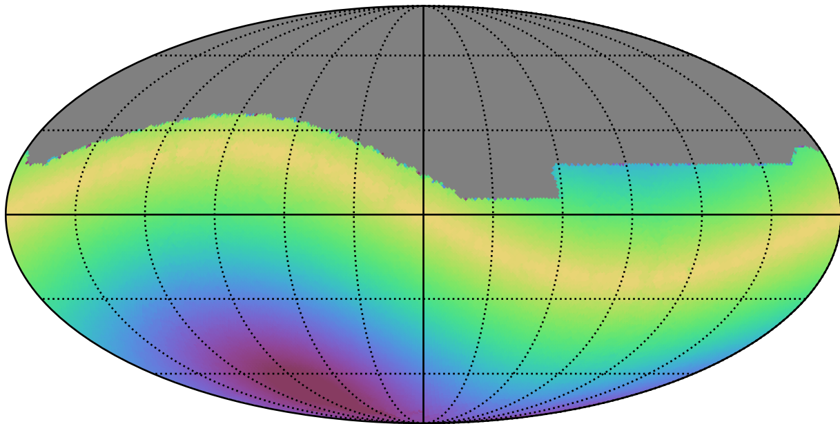
noroll_v3.4_10yrs All sky i band: Max solarElong
