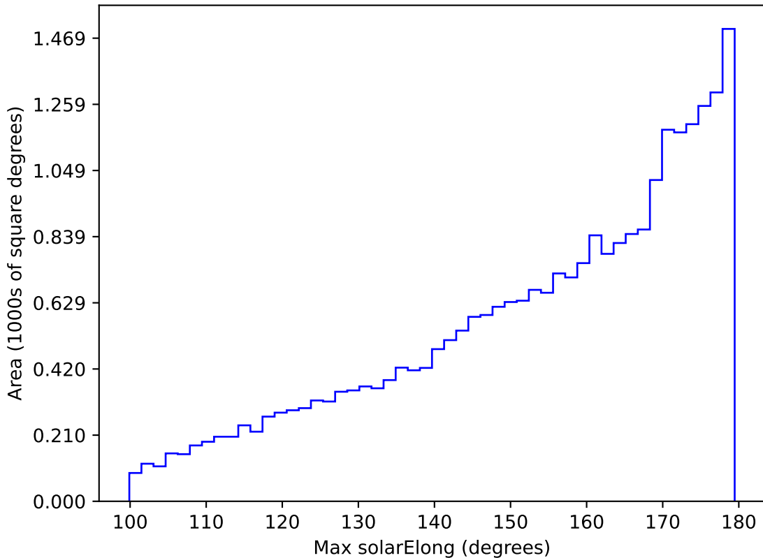
noroll_v3.4_10yrs All sky i band: Max solarElong
