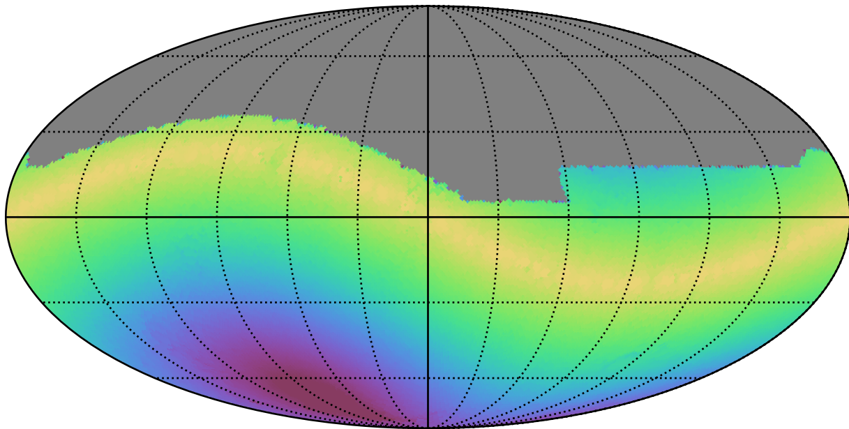
noroll_v3.4_10yrs All sky g band: Max solarElong
