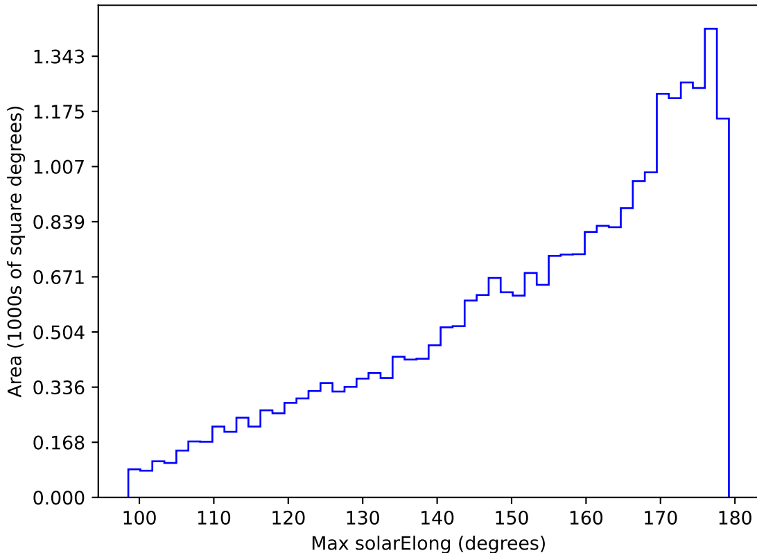
noroll_v3.4_10yrs All sky g band: Max solarElong
