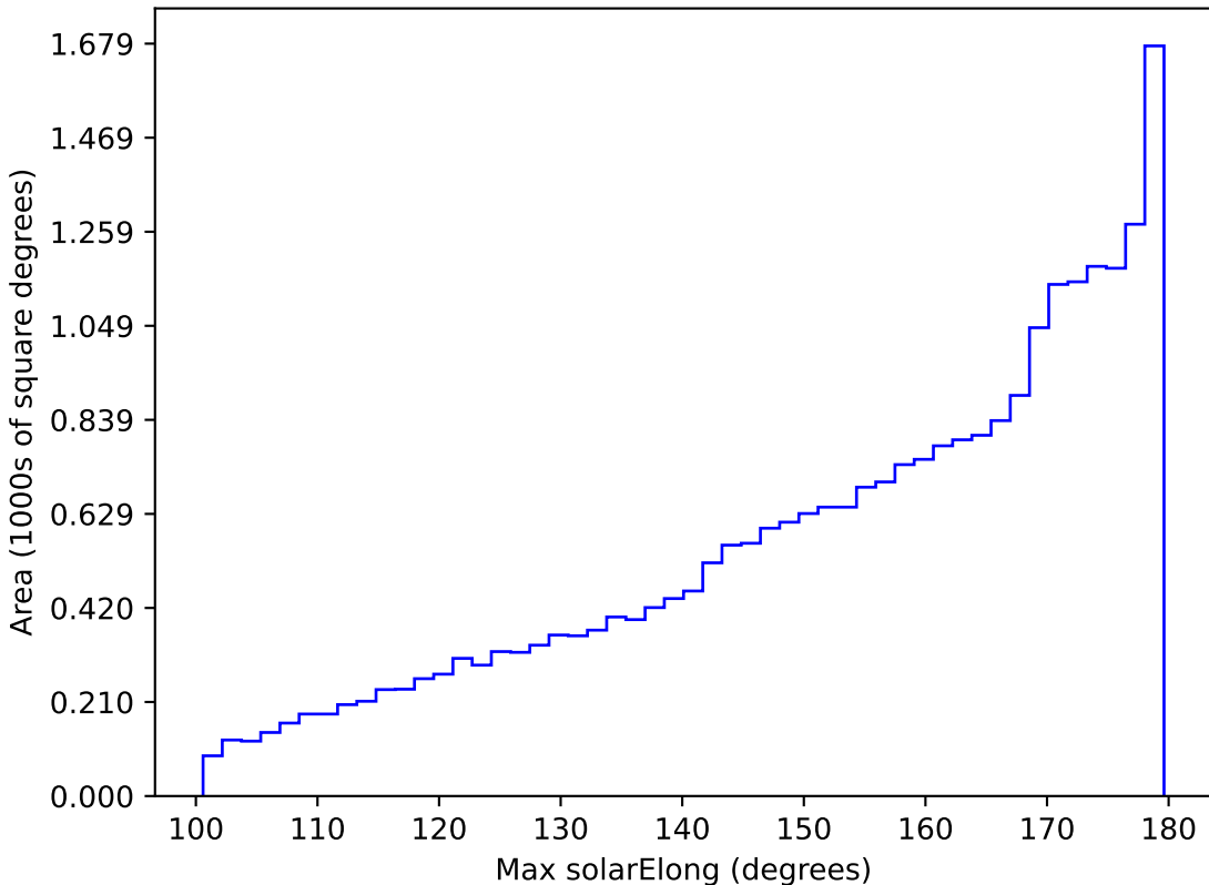
noroll_v3.4_10yrs All sky all bands: Max solarElong
