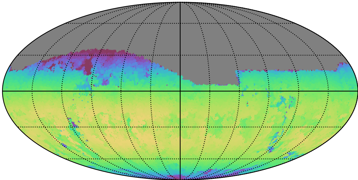
noroll_v3.4_10yrs Yr 1 z band: Max skyBrightness
