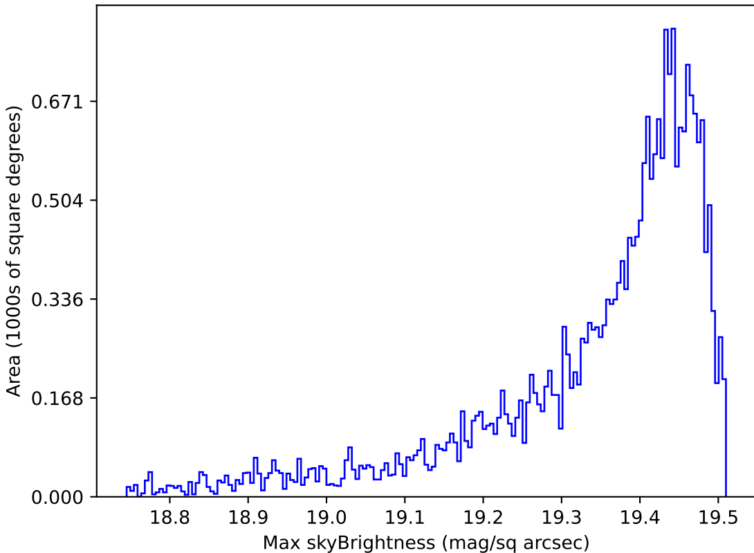
noroll_v3.4_10yrs Yr 1 z band: Max skyBrightness
