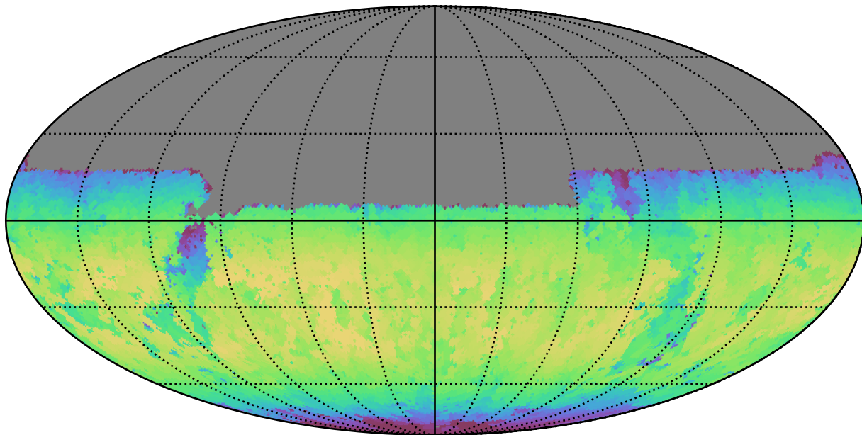
noroll_v3.4_10yrs Yr 1 y band: Max skyBrightness
