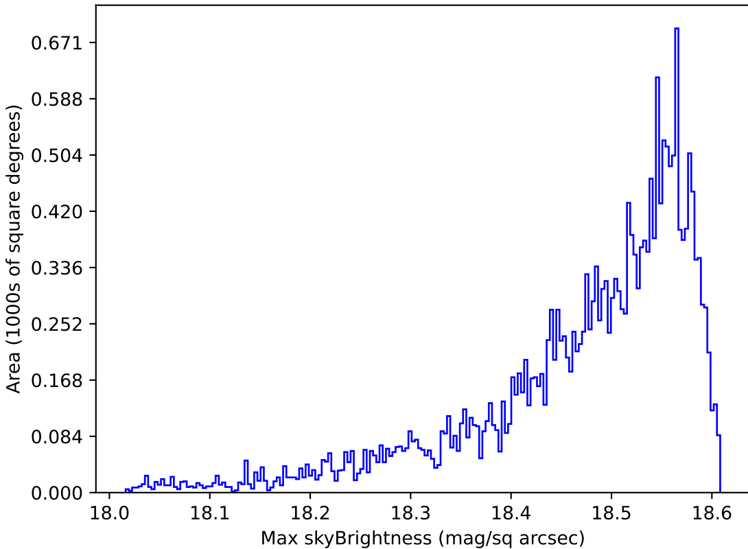
noroll_v3.4_10yrs Yr 1 y band: Max skyBrightness
