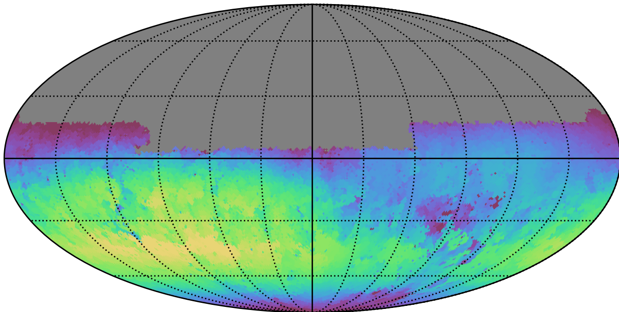
noroll_v3.4_10yrs Yr 1 u band: Max skyBrightness
