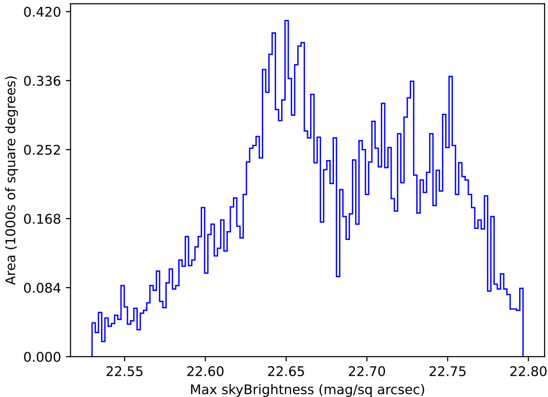
noroll_v3.4_10yrs Yr 1 u band: Max skyBrightness
