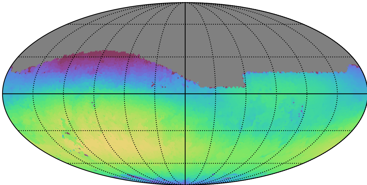
noroll_v3.4_10yrs Yr 1 r band: Max skyBrightness
