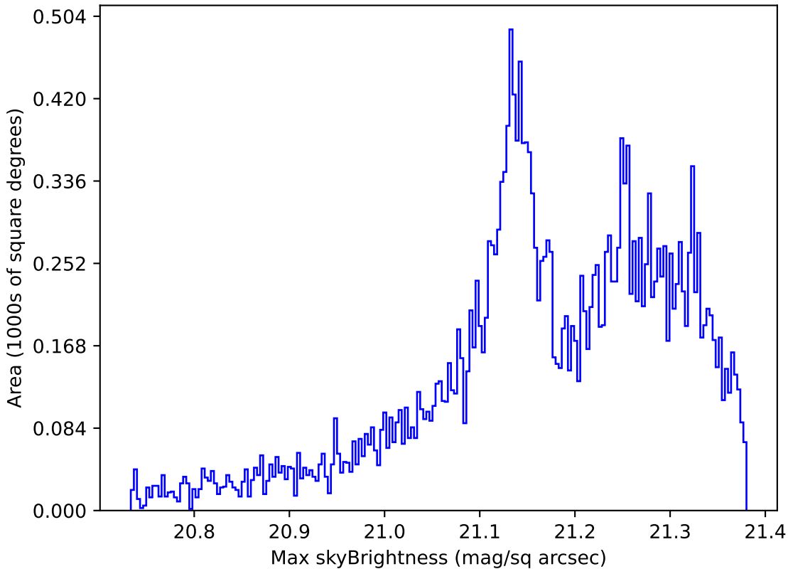
noroll_v3.4_10yrs Yr 1 r band: Max skyBrightness
