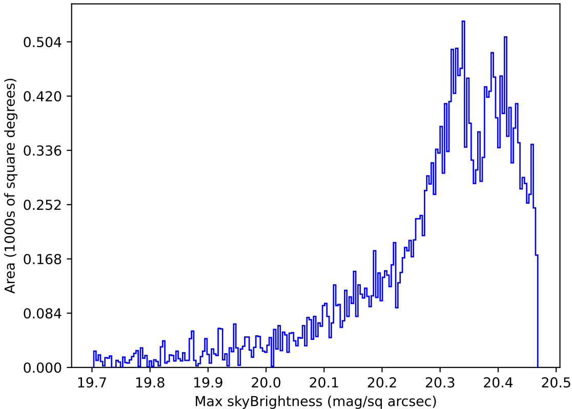
noroll_v3.4_10yrs Yr 1 i band: Max skyBrightness
