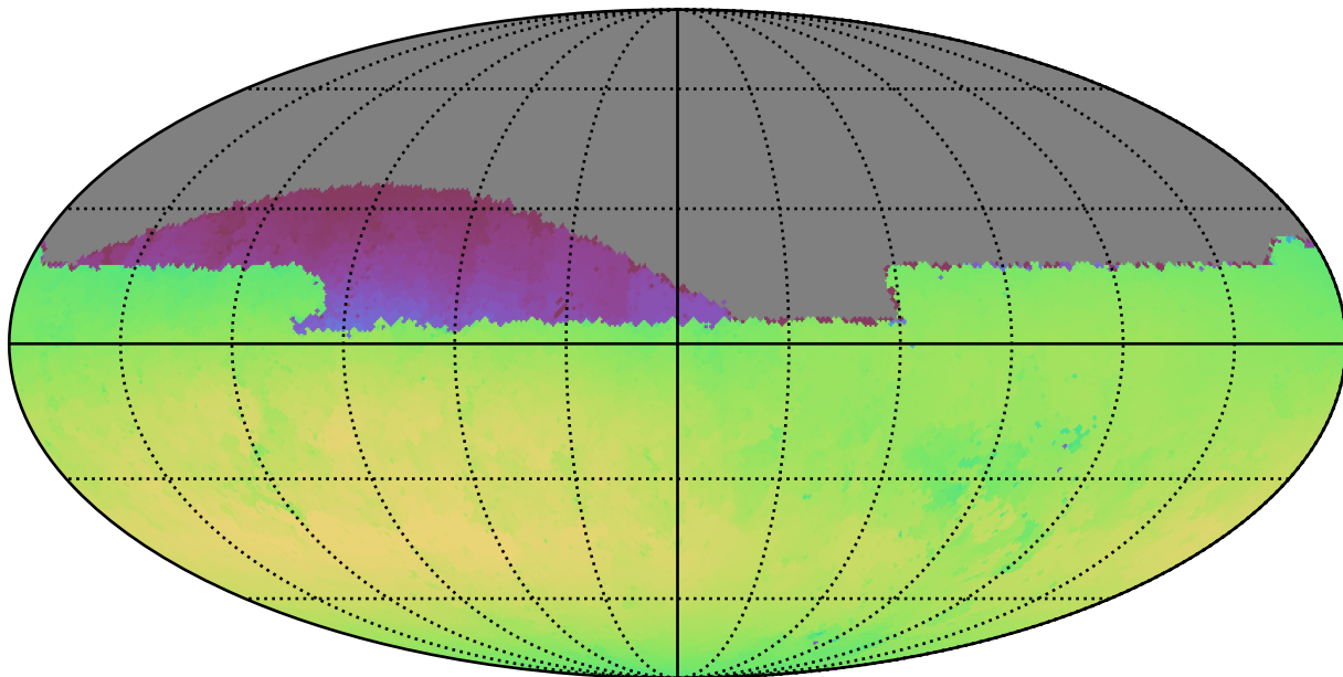
noroll_v3.4_10yrs Yr 1 all bands: Max skyBrightness
