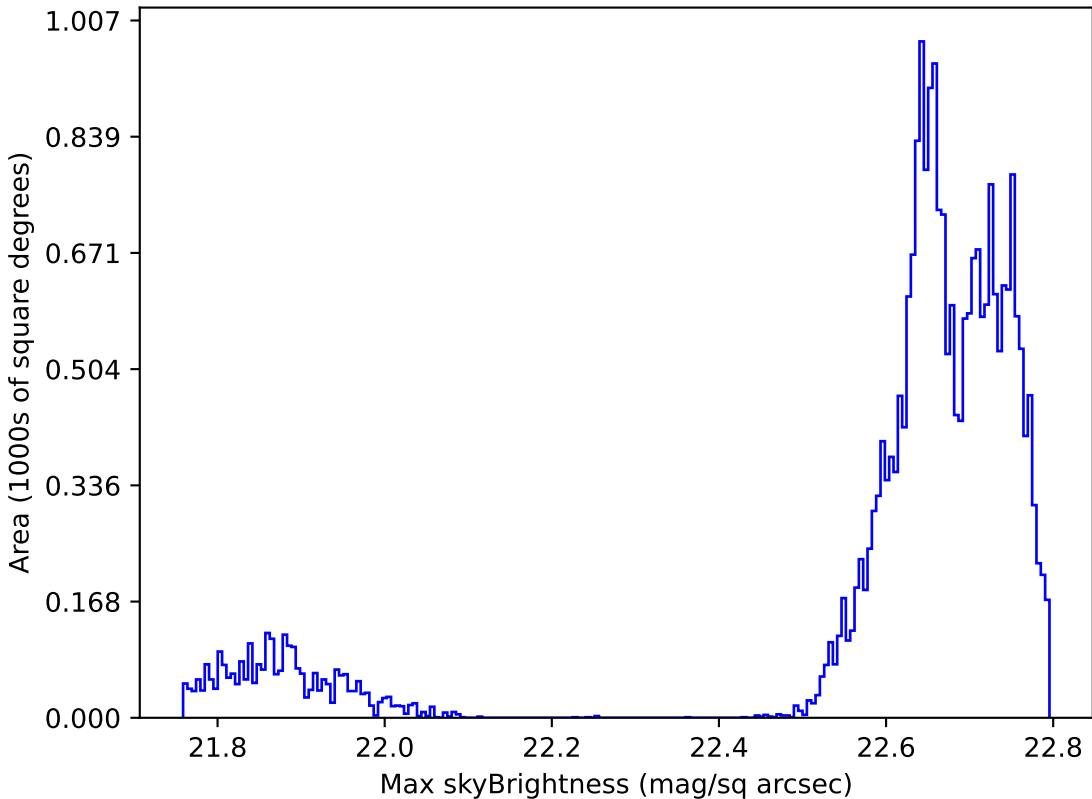
noroll_v3.4_10yrs Yr 1 all bands: Max skyBrightness
