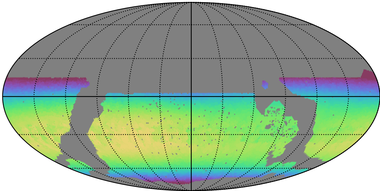
noroll_v3.4_10yrs WFD z band: Max skyBrightness
